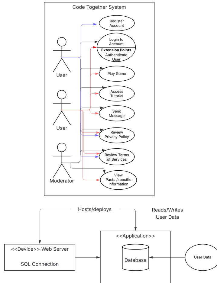
Figure 5: Use Case Diagram
