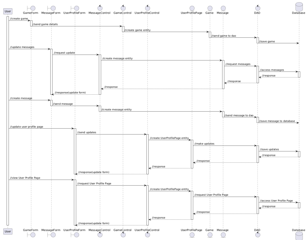
Figure 3: Application Sequence Diagram
