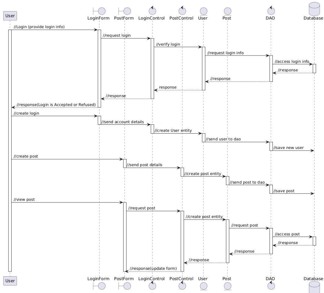
Figure 2: User Sequence Diagram
