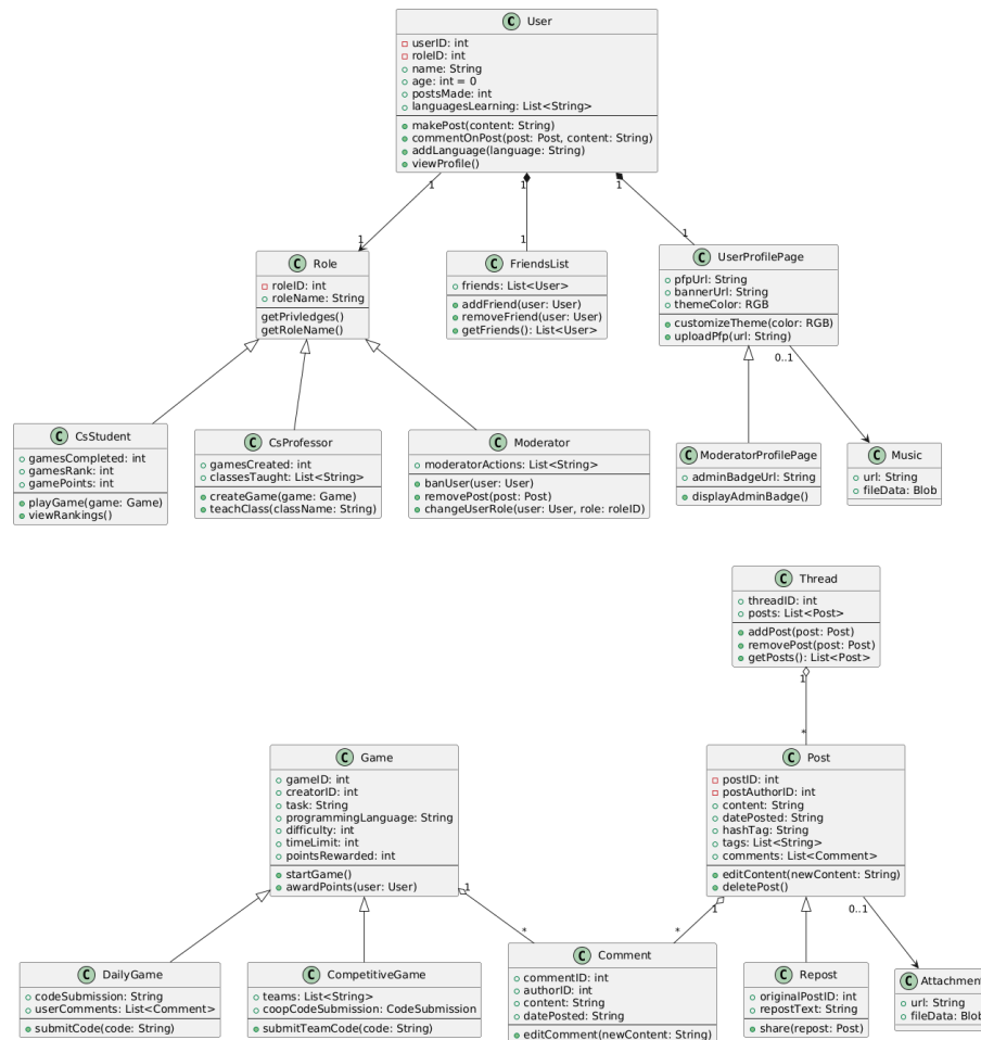
Figure 1: Class Diagram
